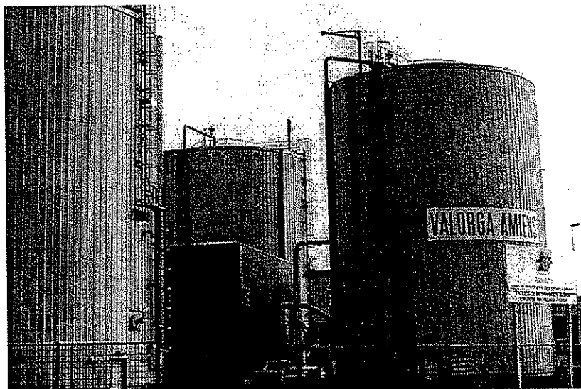
This MSW digester has operated continuously since 1988 (photo credit: Krijn Braber, NOVEM)
