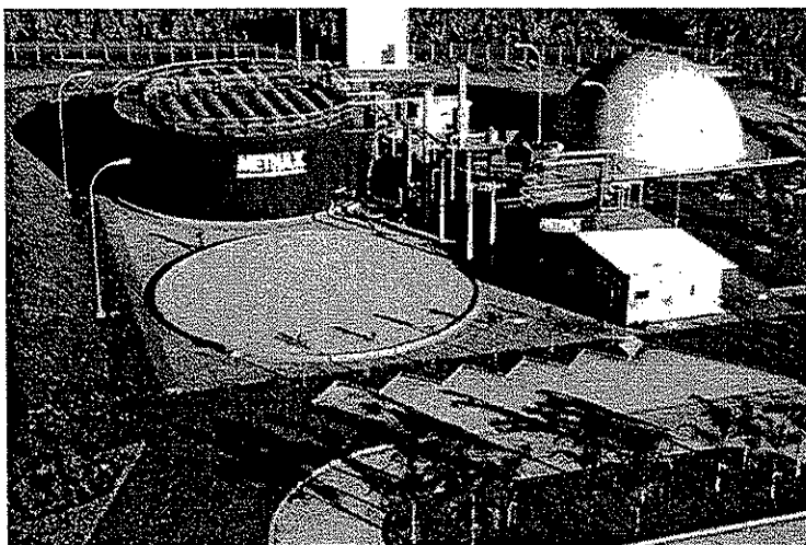
A digester treating dilute wastewater at a fuel ethanol production plant in Brazil (photo credit: Paques BV)
