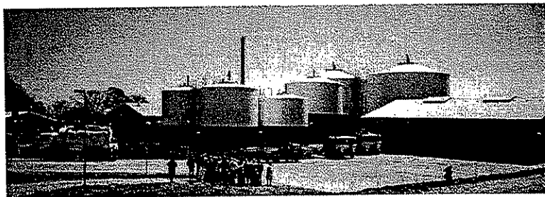
A centralized Danish digester processing manure, organic industrial residue, and biowaste
